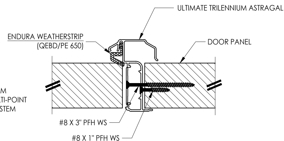
4 HORIZONTAL CROSS SECTION
